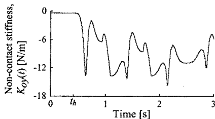
(a) Change of non-contact stiffness K_{Oy}(t)
