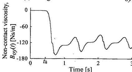
(b) Change of non-contact viscosity B_{Oy}(t)
