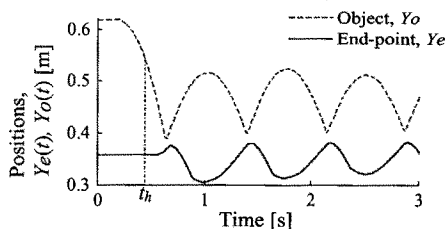
(a) Trajectories of Object and End-point with learning
