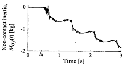
(c) Change of non-contact inertia M_{Oy}(t)
