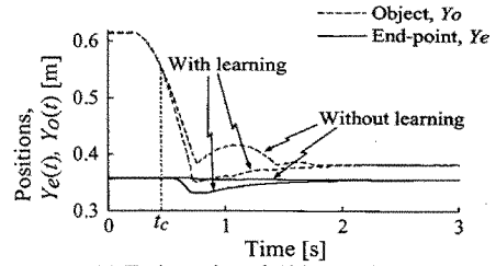
(a) Trajectories of Object and End-point with and without learning
